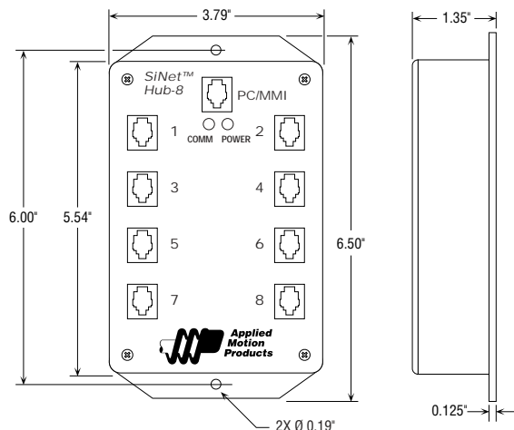
MECHANICAL OUTLINE:
