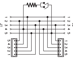
2-port Wiring Diagram
